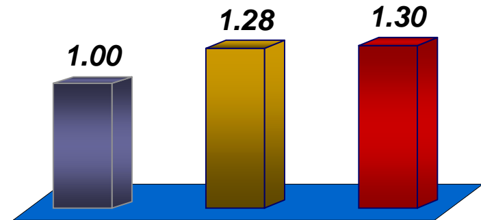
Integer SPECint_base2000
